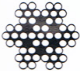
Galvanized steel wire rope 7x7 + Metal Core
